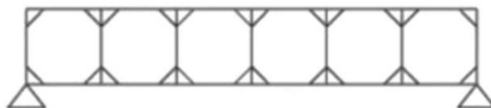
Vierendeel truss with rigid joint(stable)
